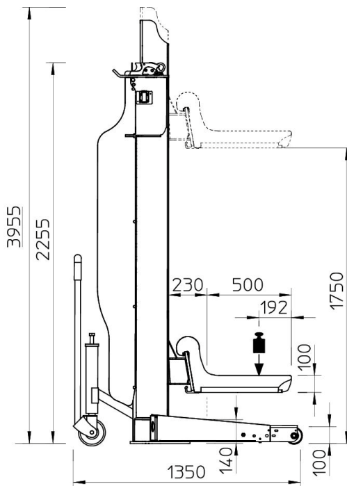
Mobile column EHB905V11DC-FEX Length of fork 500 mm
