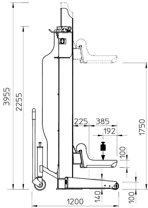
Mobile column EHB905V11DC Length of fork 385 mm
