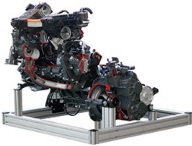
Diesel Common rail INJECTION + GEARBOX cutaway model
