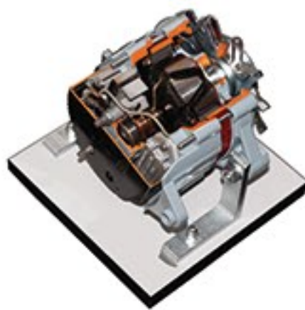
Alternator single-flow cooling Cutaway model
