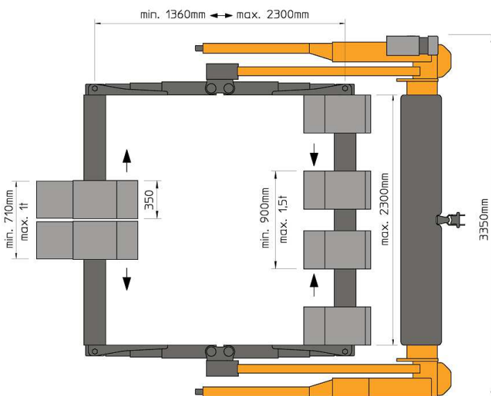
Pic. FHB3000-SS-2300 with ascending device FA-TORO
