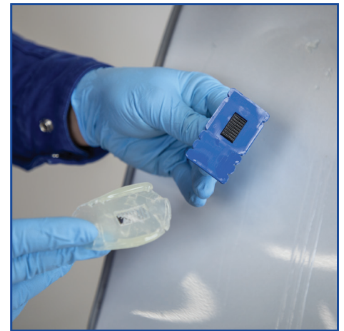
Plastic tabs are reusable and ready to pull dent after dent.
