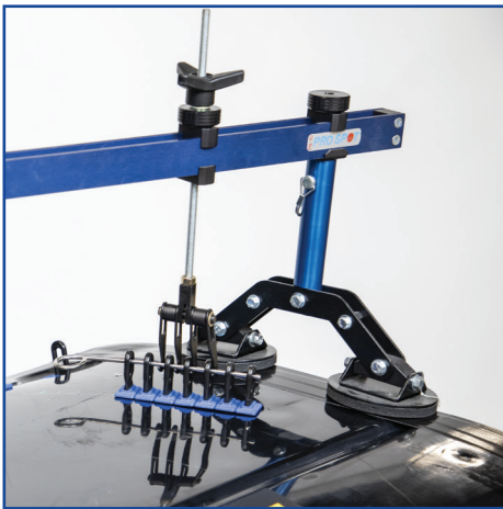
Quickly remove dents when paired with the PB-10 Pull Bar.
