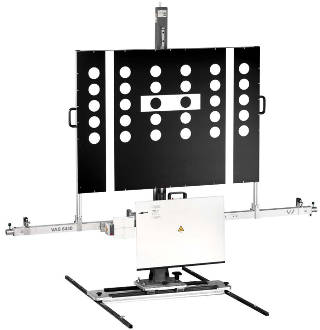
VAS 6430 with rail system VAS 6430/7
